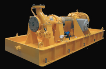
OH2 SEALLESS MAGNETIC DRIVE, CENTERLINE MOUNTED, SINGLE STAGE OVERHUNG IMPELLER PUMPS • Separation • Process • Scrubbing • H 2 S Removal
